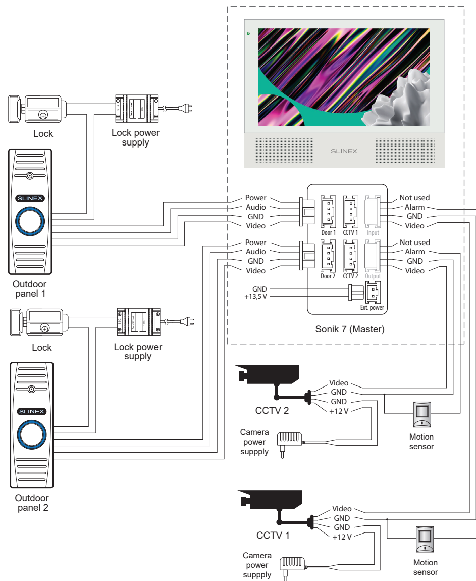
Diagram 1. Sonik 7 outdoor panels, cameras and locks connection.
