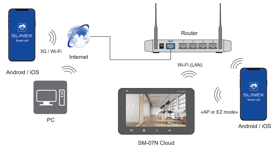
Diagram 2. SM-07N Cloud wireless Wi-Fi network connection.
